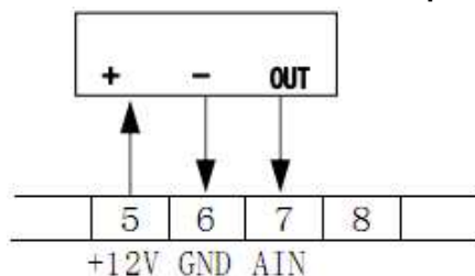
G. Three wire current modulated pulse sensor
