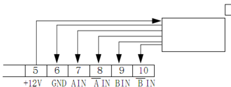
F. Line receiver input
