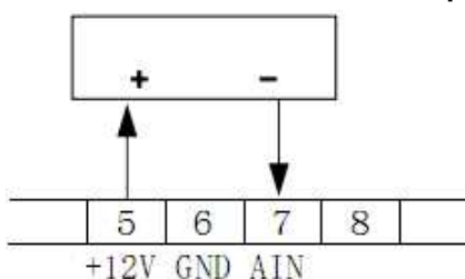
H. Two wire current modulated pulse sensor
